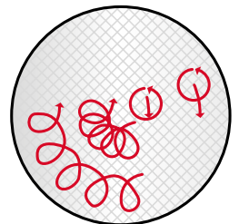
Figure 36b. Random orbital
